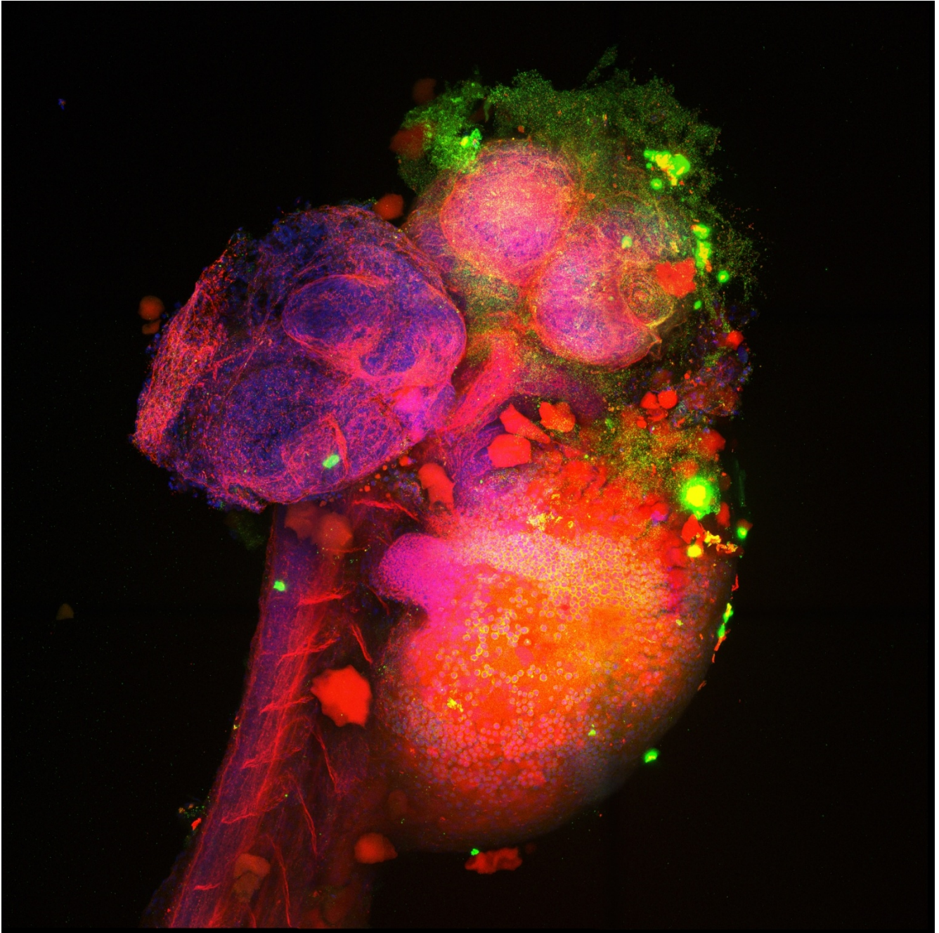
Flat view of a 3D-reconstructed zebrafish tissue sample, where each fluorescent marker indicates a different protein.
